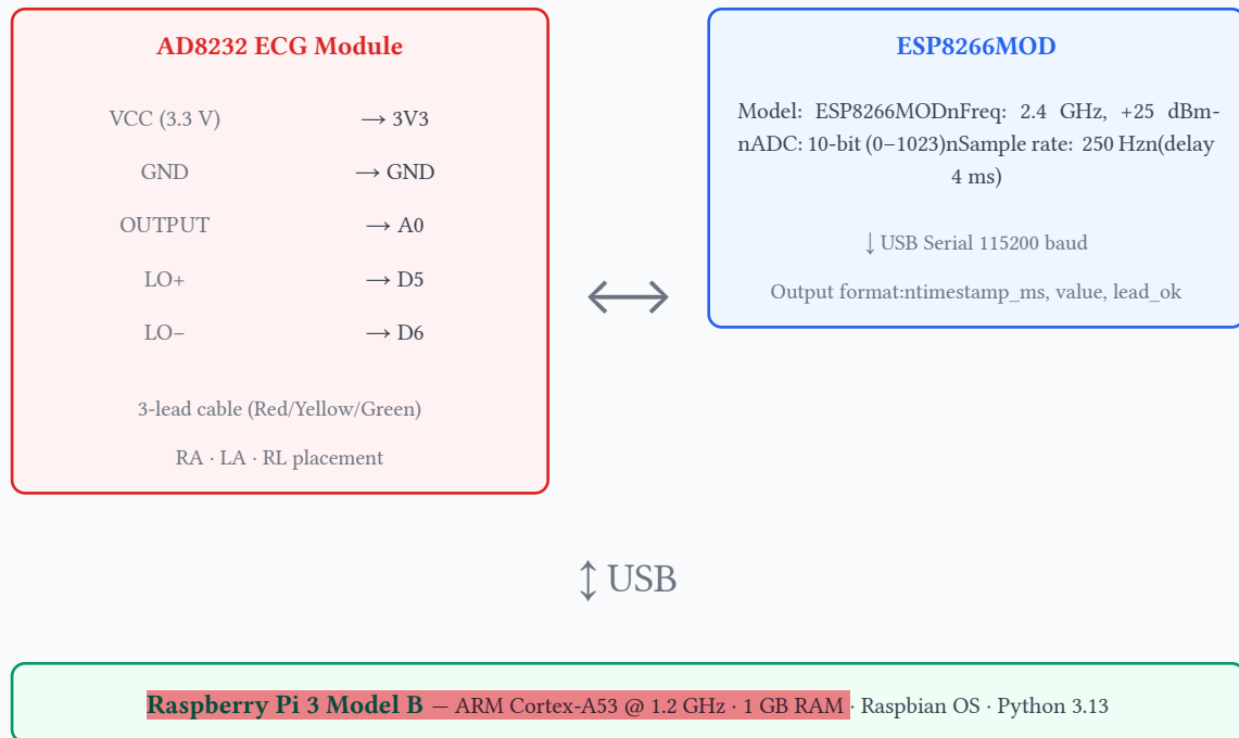
Figure 2: Hardware Connection Diagram
